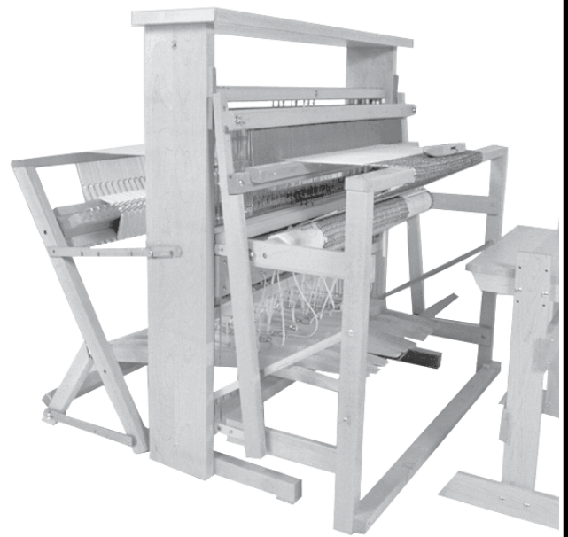
Treadles with rockers
